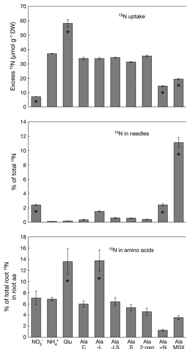
Fig. 1. Top panel displays total uptake of N sources. Middle panel shows relative distribution of total ^{15}\text{N} into needles (as calculated by ^{15}\text{N} needles/ ^{15}\text{N} needles + ^{15}\text{N} roots). Bottom panel shows the relative amount of ^{15}\text{N} in amino acids of total root ^{15}\text{N} content. All values presented are means \pm SE ( n=3 ). Bars labelled with an asterisk exhibit significant differences from Ala controls ( P < 0.01 ). Abbreviations as in Table 1.
