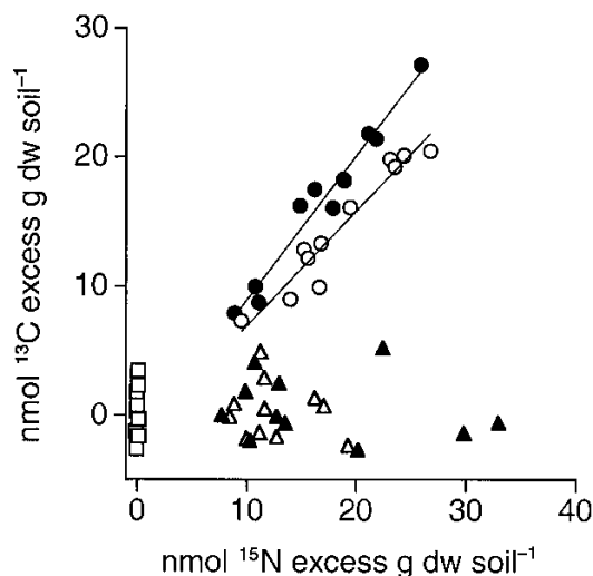
Fig. 2 The relationship between ^{15}\text{N} and ^{13}\text{C} labelling of sieved soil treated with either ^{15}\text{NH}_4^+ (closed triangles); ^{15}\text{NO}_3^- (open triangles); U- ^{13}\text{C}_2 , [ ^{15}\text{N} ]-glycine (closed circles); 2- ^{13}\text{C} , [ ^{15}\text{N} ]-glycine (open circles) or water only (open squares). Each symbol represents one soil sample. Lines indicate linear regression for U- ^{13}\text{C}_2 , [ ^{15}\text{N} ]-glycine ( y = 1.11x - 2.16 , r^2 = 0.96 ), and for 2- ^{13}\text{C} , [ ^{15}\text{N} ]-glycine ( y = 0.88x - 1.86 , r^2 = 0.93 ), P < 0.001 for both.
