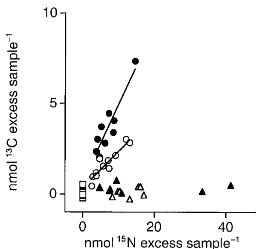
Fig. 1 The relationship between excess ^{15}\text{N} and excess ^{13}\text{C} of root extracts of field grown wheat plants supplied with either ^{15}\text{NH}_4^+ (closed triangles); ^{15}\text{NO}_3^- (open triangles); U- ^{13}\text{C}_2 , ^{15}\text{N} -glycine (closed circles) or 2- ^{13}\text{C} , ^{15}\text{N} -glycine (open circles) or water only (open squares) through the soil. (Each symbol represents one analysis of a root extract from 8 to 10 plants.) Lines indicate linear regression for U- ^{13}\text{C}_2 , ^{15}\text{N} -glycine ( y = 0.43x + 0.7 , r^2 = 0.86 ) and for 2- ^{13}\text{C} , ^{15}\text{N} -glycine ( y = 0.20x + 0.3 , r^2 = 0.84 ), P < 0.001 for both. For data on roots and shoots before extraction see Table 1.
